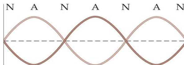
Figure 1b. A third harmonic standing wave.
